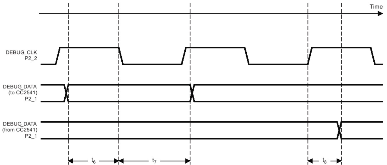
Figure 7 Slave Timing
